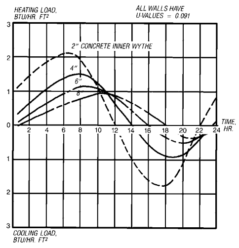
(c) CONCRETE SANDWICH WALLS
