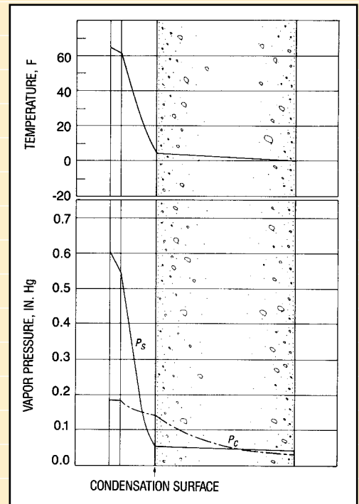
Fig. 31 – Thermal and water vapor gradients for extreme winter conditions
