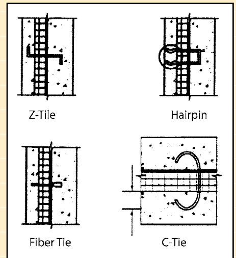
Fig. 42 – Tension/compression ties
