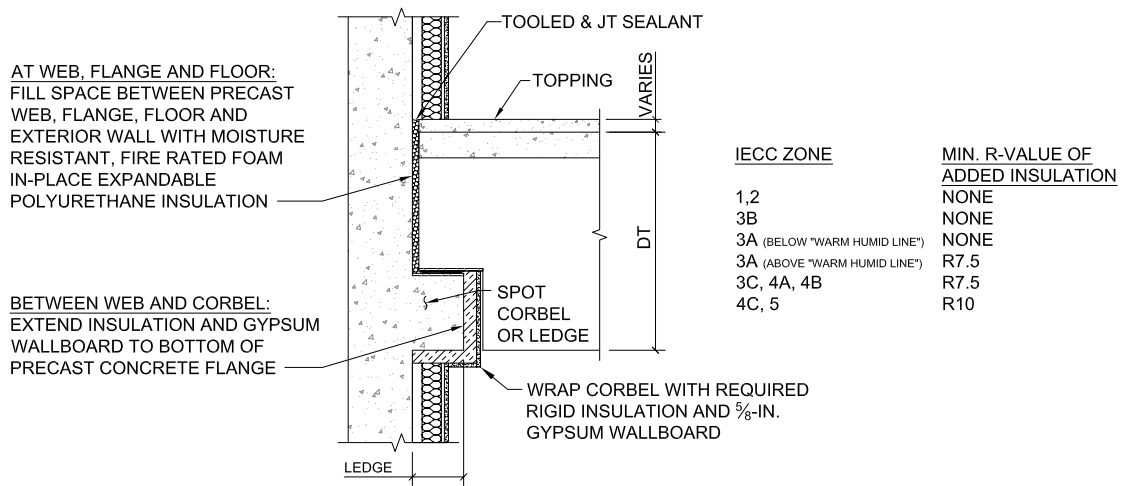
C PRECAST CONCRETE WITH BATT INSULATION NTS
