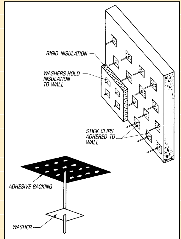
Fig. 33 – Use of stick clips to install rigid insulation
