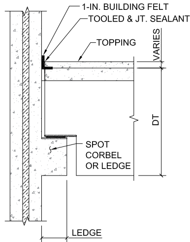
A PRECAST SANDWICH PANEL WALL NTS
