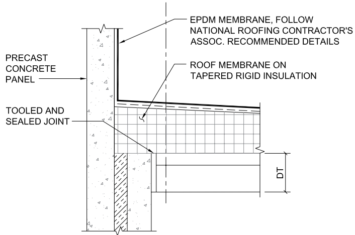
A PRECAST SANDWICH PANEL WALL NTS
