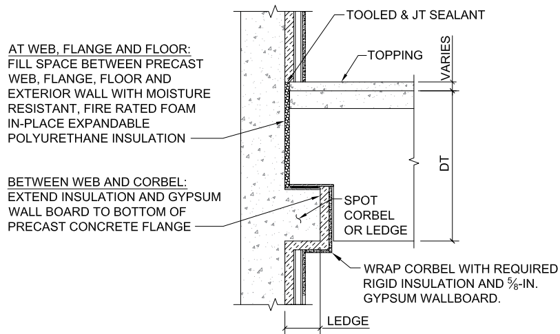
B PRECAST CONCRETE WITH RIGID INSULATION NTS
