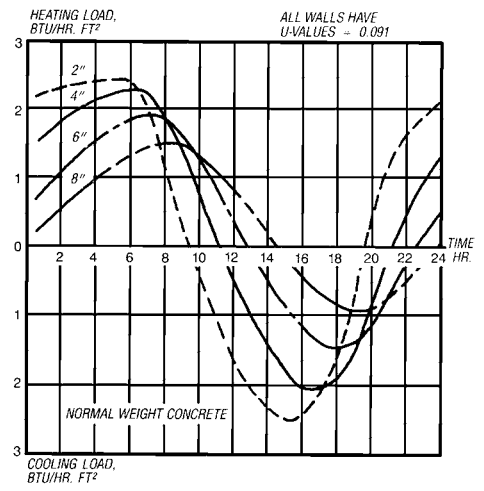
(b) CONCRETE WALLS
