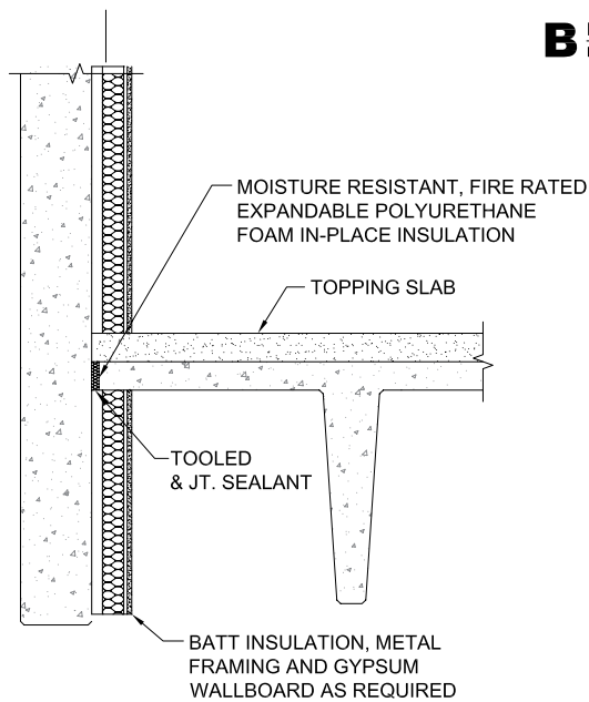
C PRECAST CONCRETE WITH BATT INSULATION NTS
