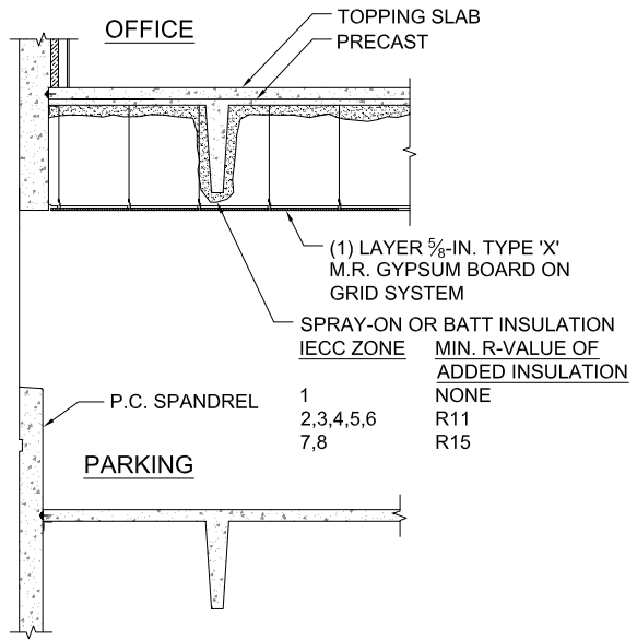
B PRECAST CONCRETE WITH RIGID INSULATION NTS
