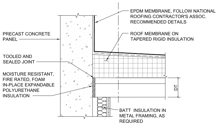
C PRECAST CONCRETE WITH BATT INSULATION NTS
