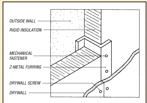
Fig. 34 – Furring systems
