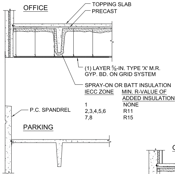
A PRECAST SANDWICH PANEL WALL NTS
