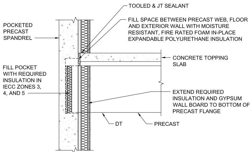
Fig. 29 – Typical Pocketed Loadbearing Spandrel/DT Detail
