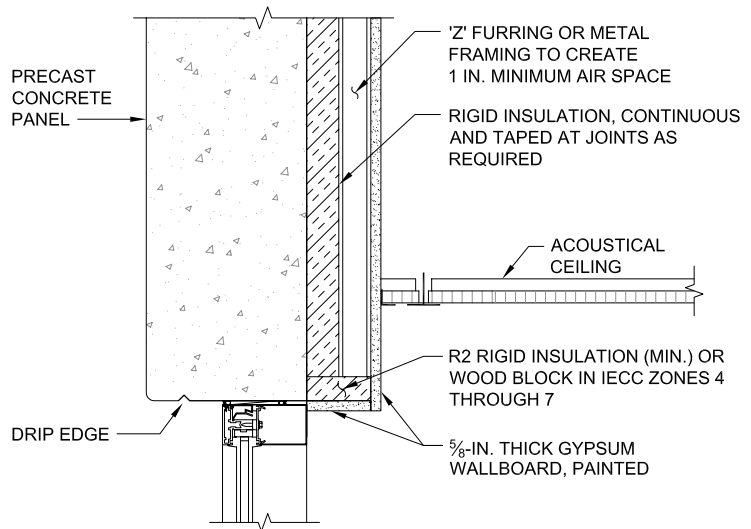
B PRECAST CONCRETE WITH RIGID INSULATION NTS
