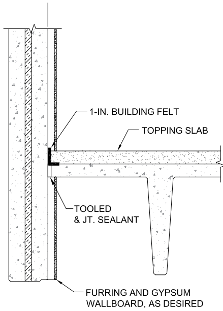
A PRECAST SANDWICH PANEL WALL NTS
