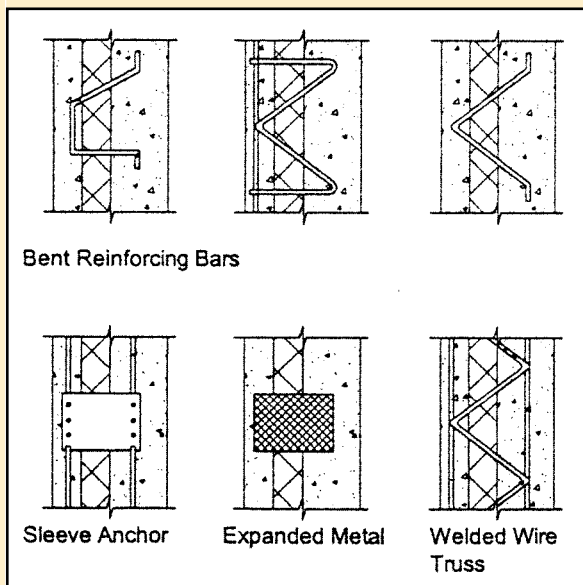
Fig. 41 – Typical shear connections
