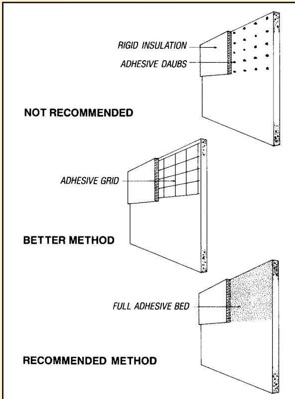
Fig. 32— Application of rigid insulation with adhesives
