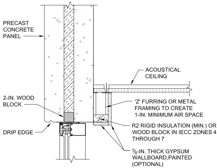
A PRECAST SANDWICH PANEL WALL NTS
