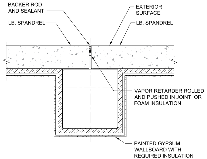
B PRECAST CONCRETE WITH RIGID INSULATION NTS
