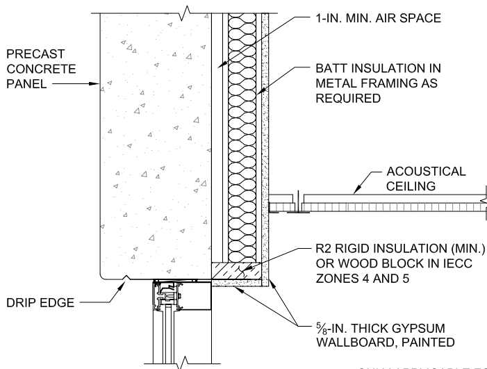
C PRECAST CONCRETE WITH BATT INSULATION NTS
