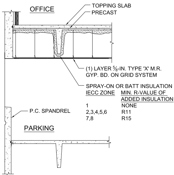
C PRECAST CONCRETE WITH BATT INSULATION NTS
