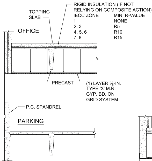
A PRECAST SANDWICH PANEL WALL NTS
