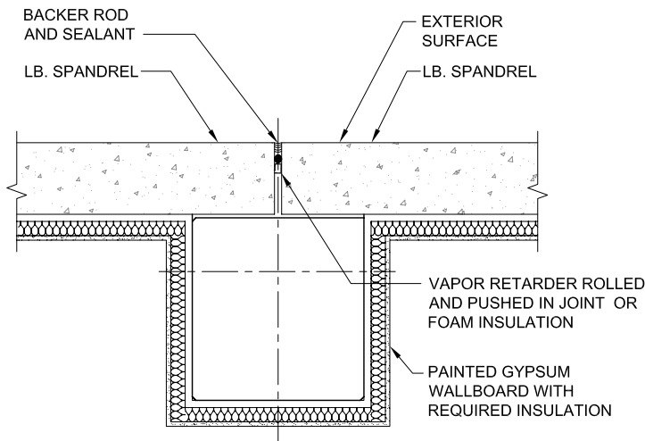
B PRECAST CONCRETE WITH RIGID INSULATION NTS
