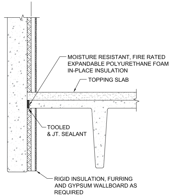
B PRECAST CONCRETE WITH RIGID INSULATION NTS
