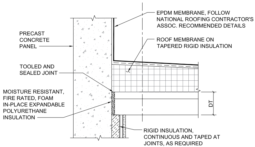
B PRECAST CONCRETE WITH RIGID INSULATION NTS
